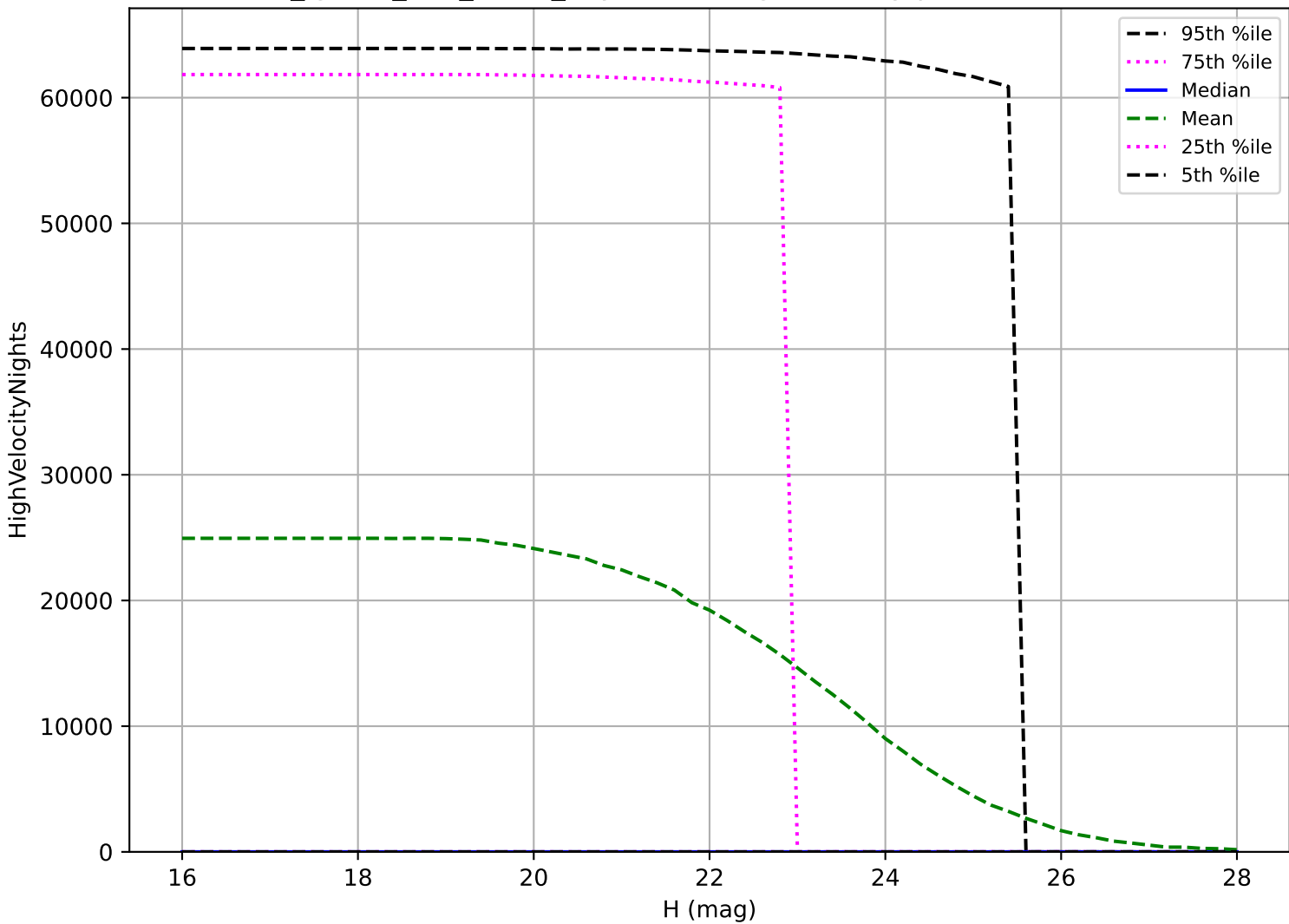
too_ignore_100_1v3.4_10yrs: PHA High velocity pair detection loss
