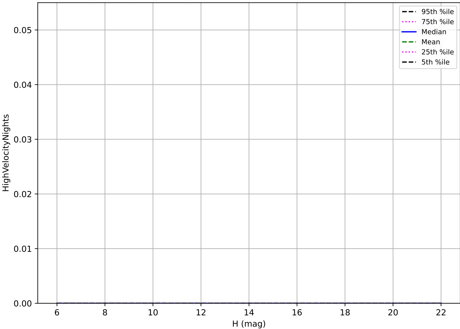
too_ignore_100_1v3.4_10yrs: OCC_r5 High velocity pair detection loss
