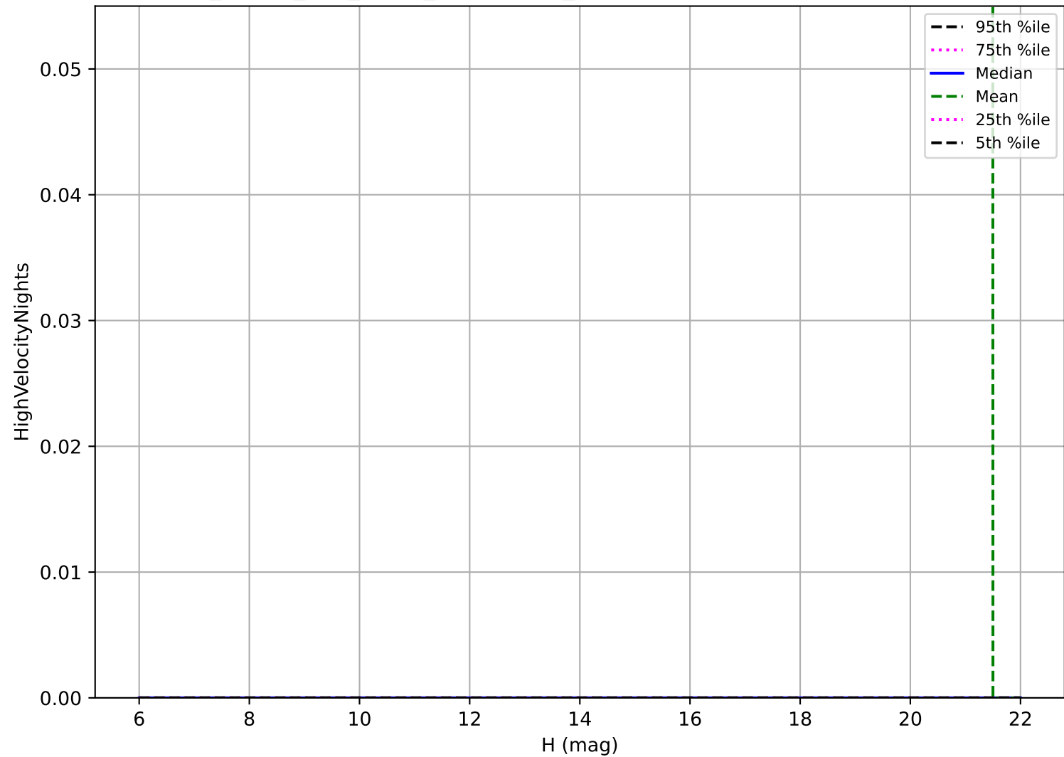
too_ignore_100_1v3.4_10yrs: OCC_r20 High velocity pair detection loss
