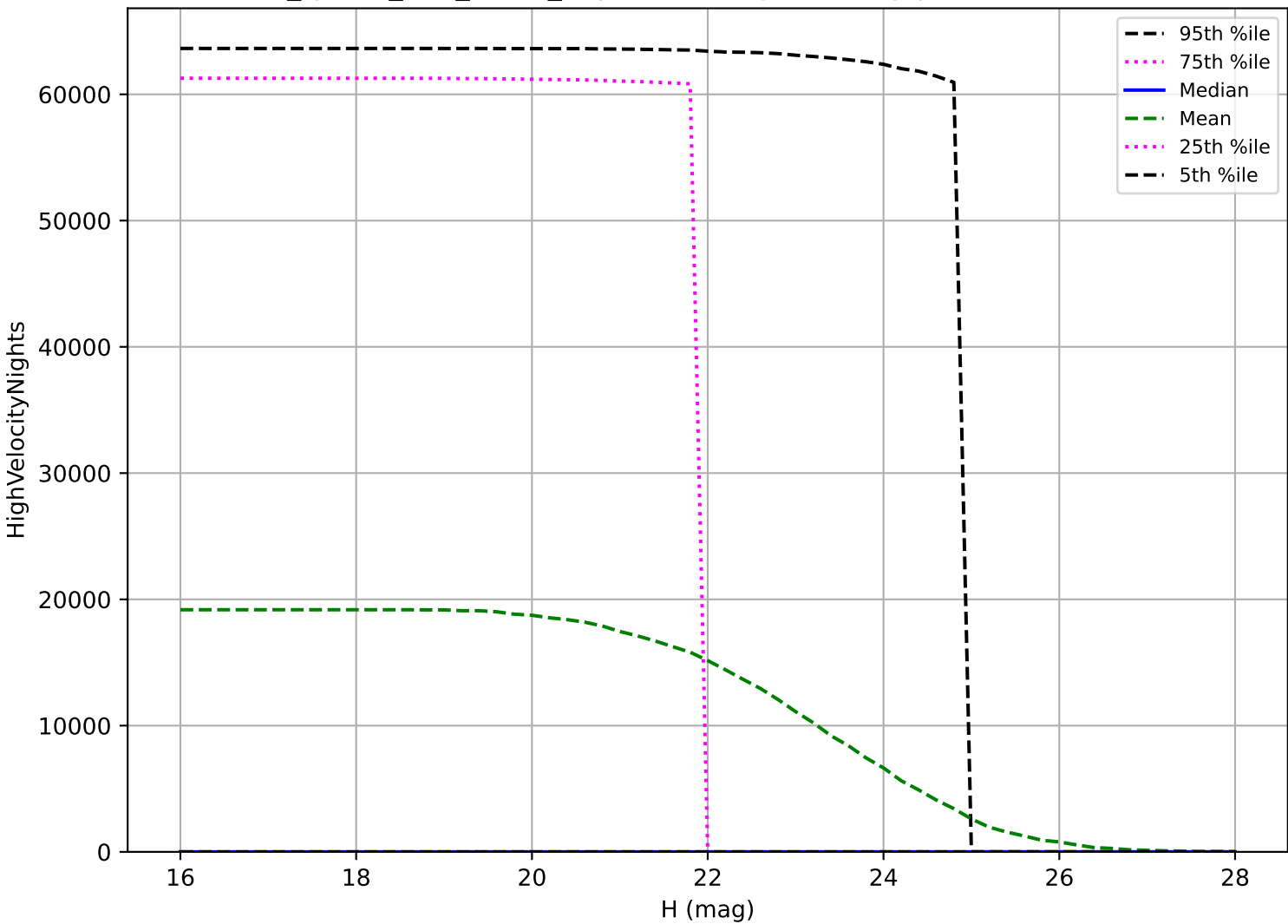
too_ignore_100_1v3.4_10yrs: NEO High velocity pair detection loss
