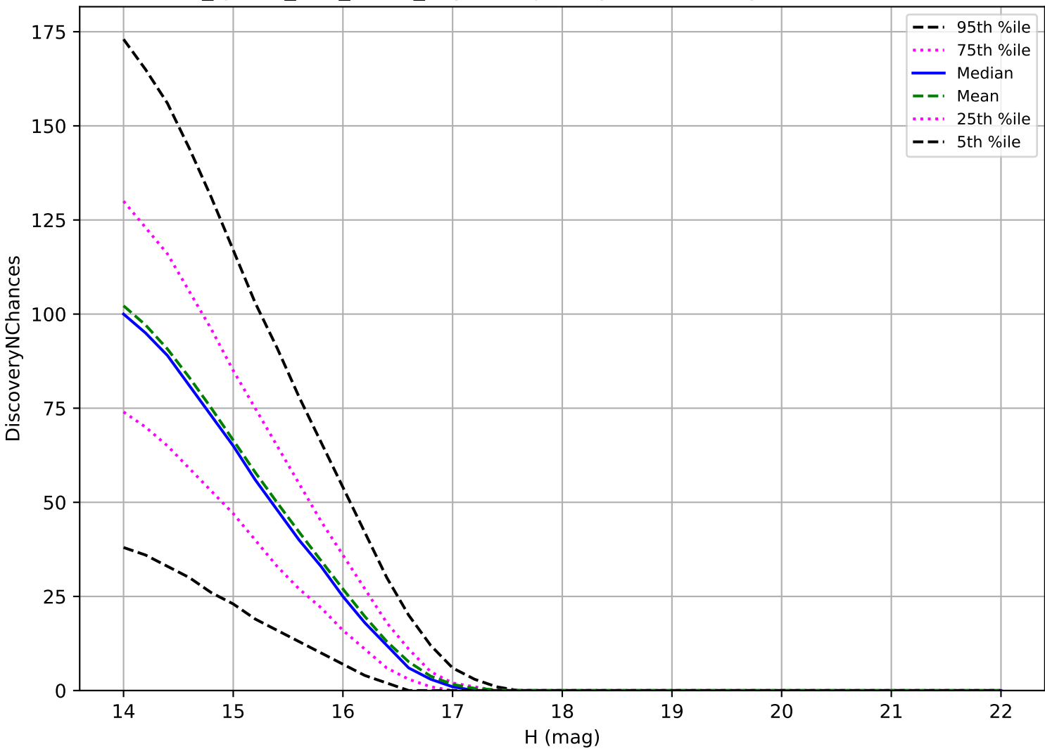
too_ignore_100_1v3.4_10yrs: Trojan 3 pairs in 15 nights detection loss
