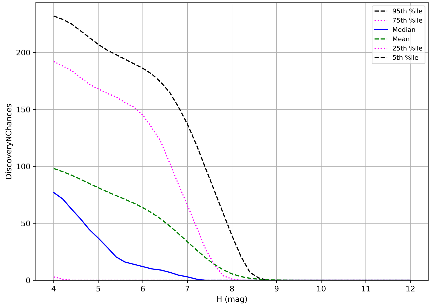
too_ignore_100_1v3.4_10yrs: TNO 3 pairs in 15 nights detection loss
