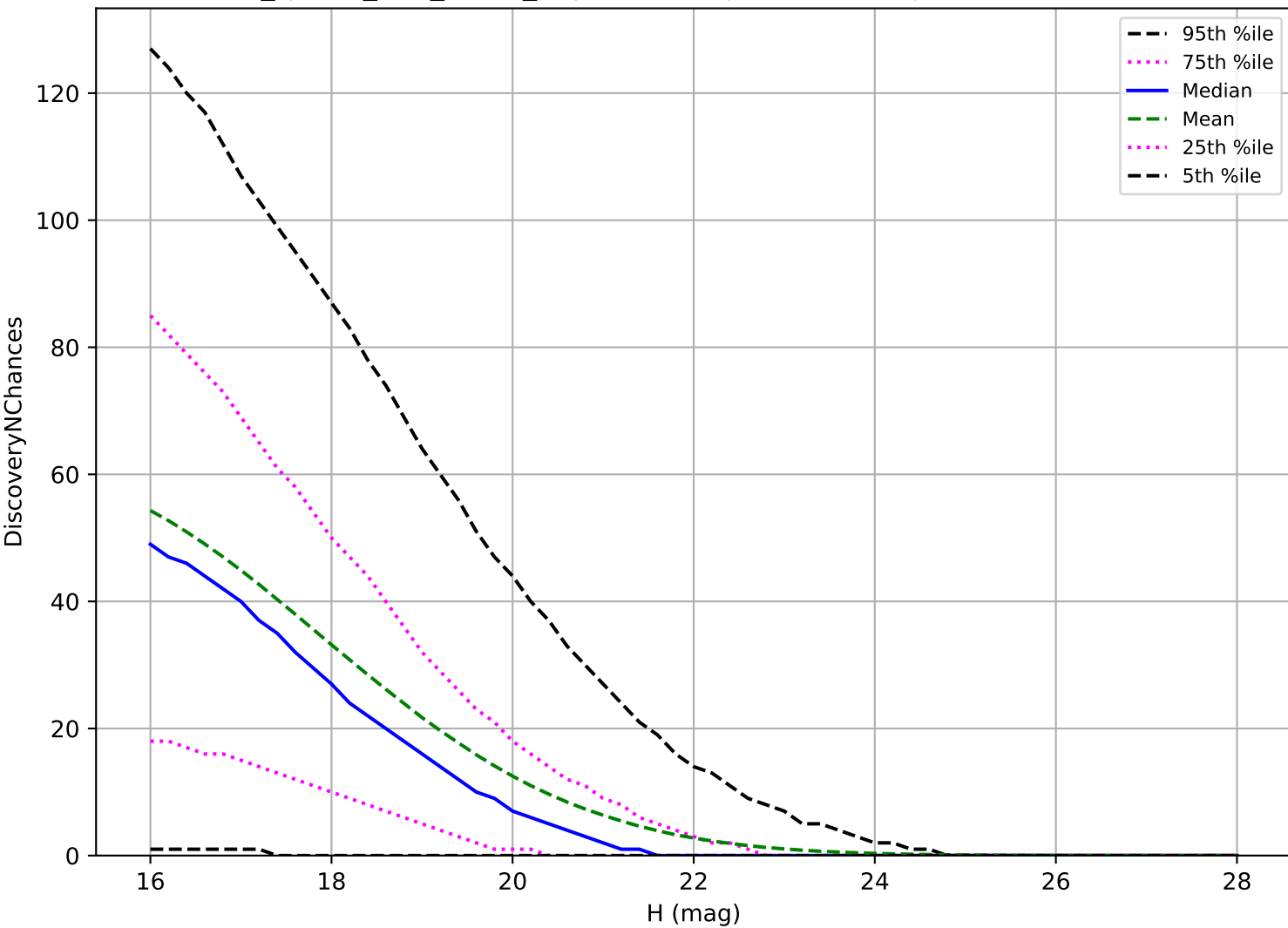
too_ignore_100_1v3.4_10yrs: PHA 3 pairs in 15 nights detection loss
