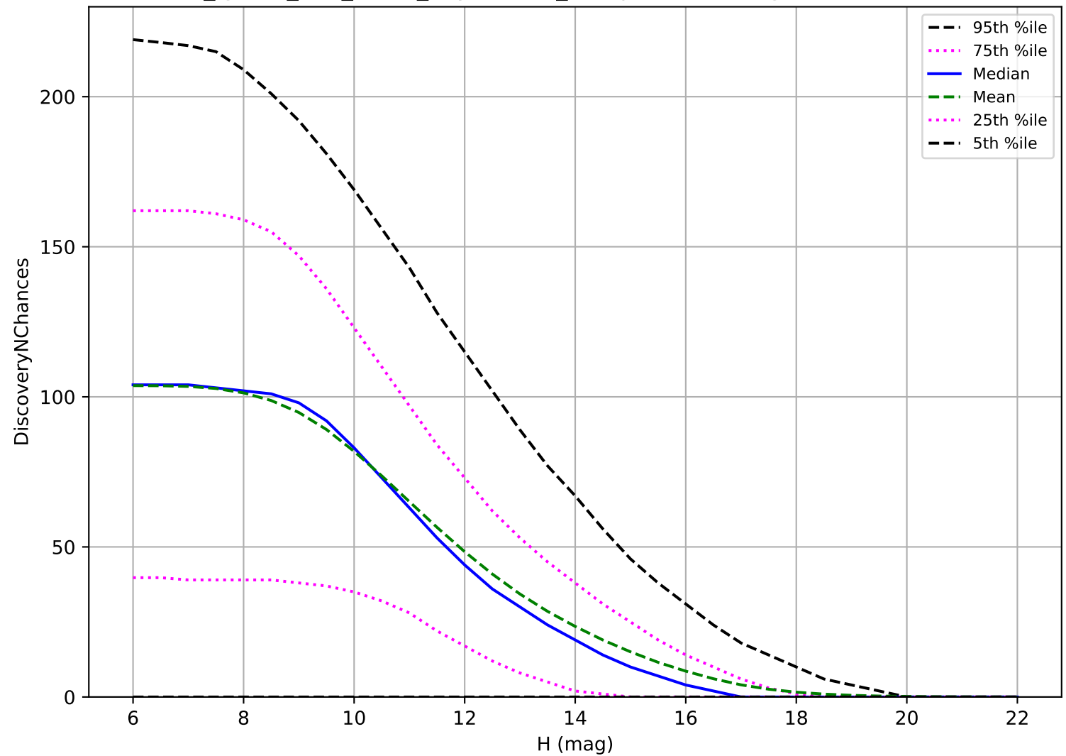
too_ignore_100_1v3.4_10yrs: OCC_r5 3 pairs in 15 nights detection loss
