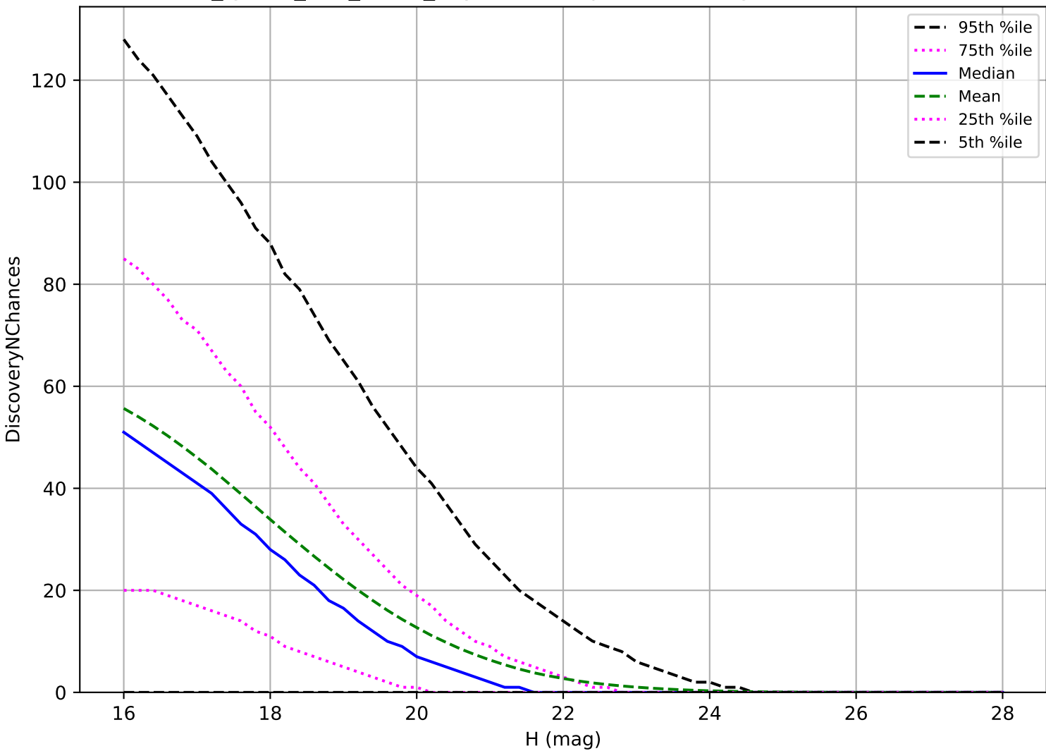
too_ignore_100_1v3.4_10yrs: NEO 3 pairs in 15 nights detection loss
