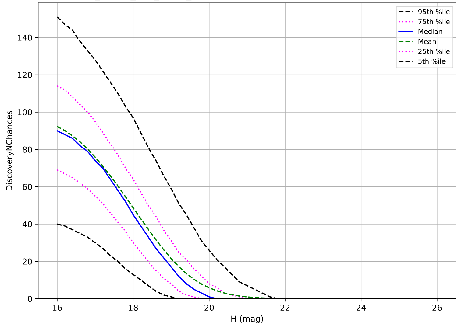
too_ignore_100_1v3.4_10yrs: MBA 3 pairs in 15 nights detection loss
