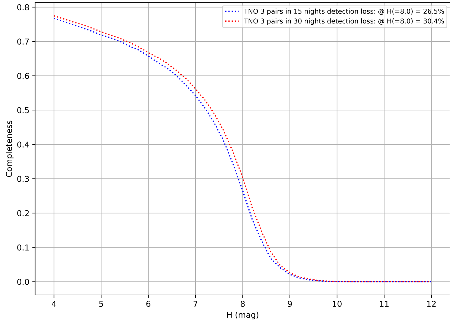
too_ignore_100_1v3.4_10yrs: DifferentialCompleteness
