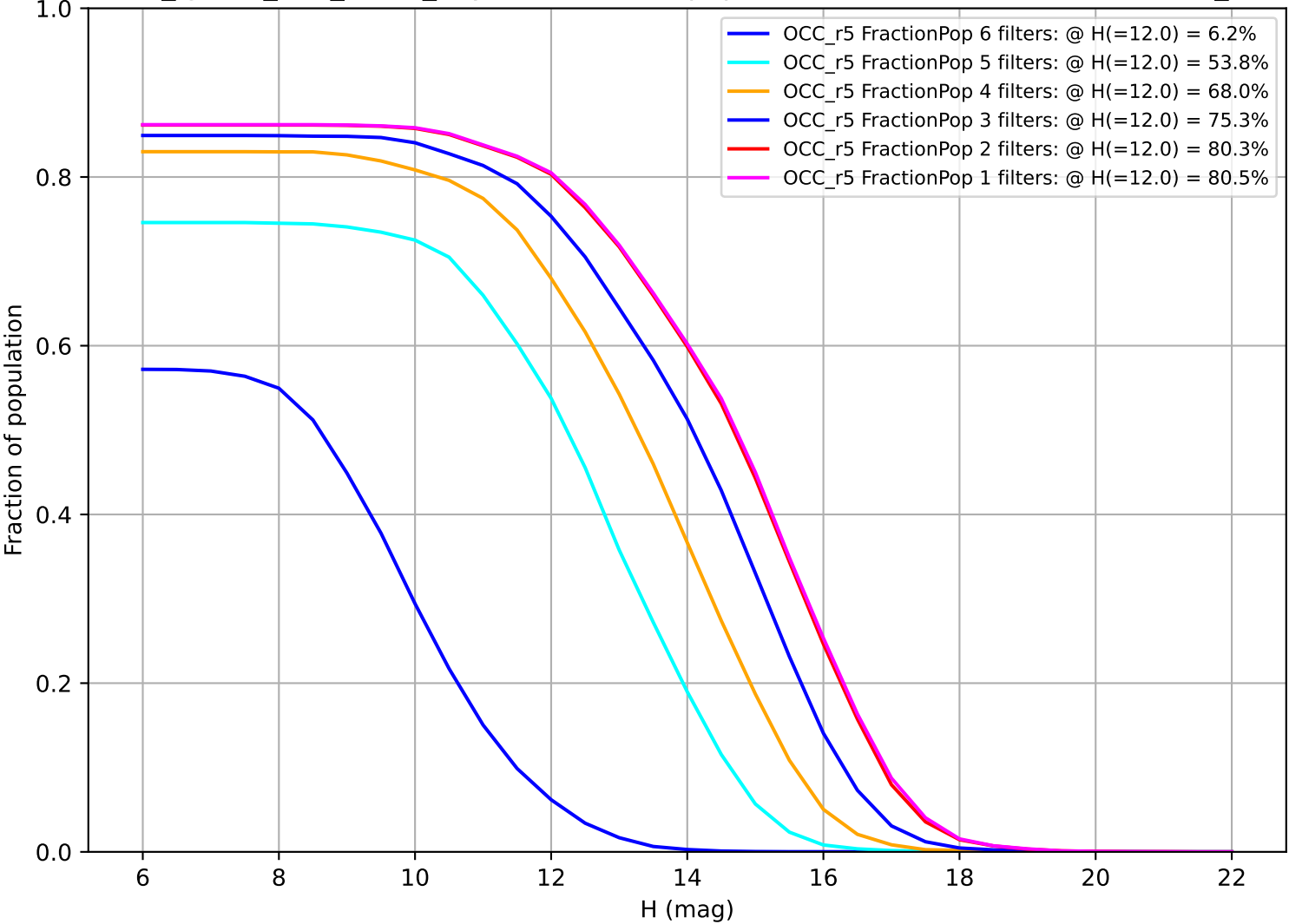
too_ignore_100_1v3.4_10yrs: Fraction of population with colors in X filters OCC_r5
