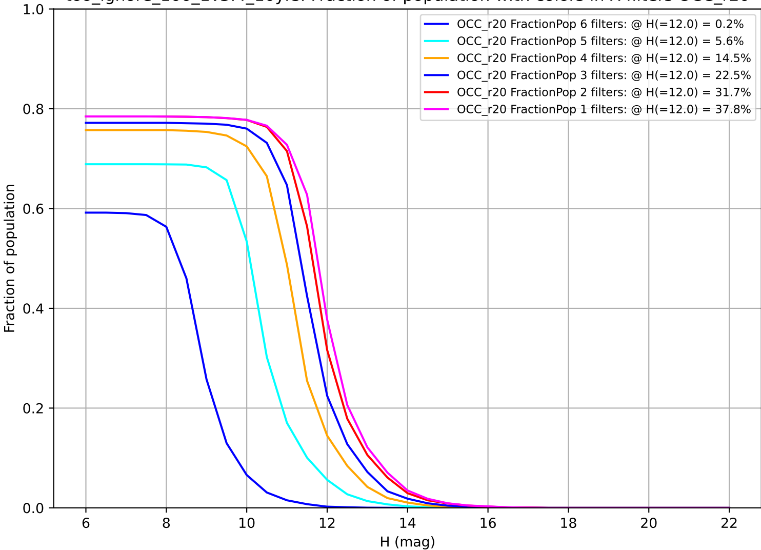
too_ignore_100_1v3.4_10yrs: Fraction of population with colors in X filters OCC_r20
