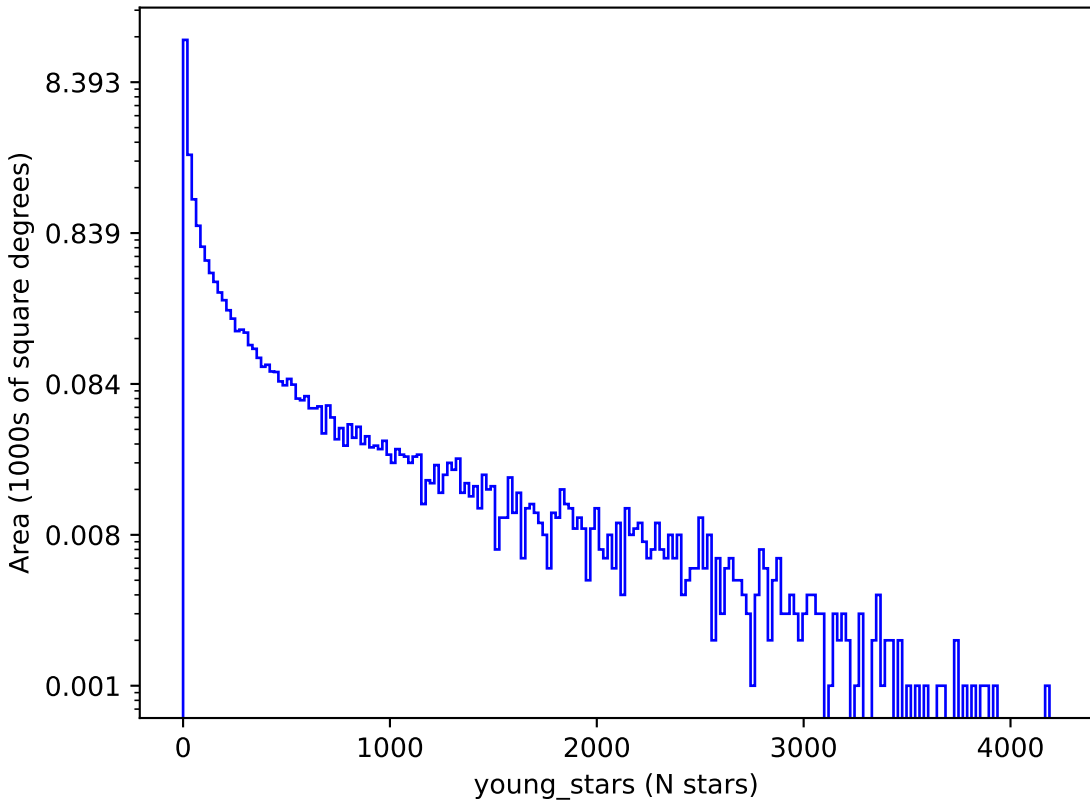
too_ignore_100_1v3.4_10yrs : young_stars
