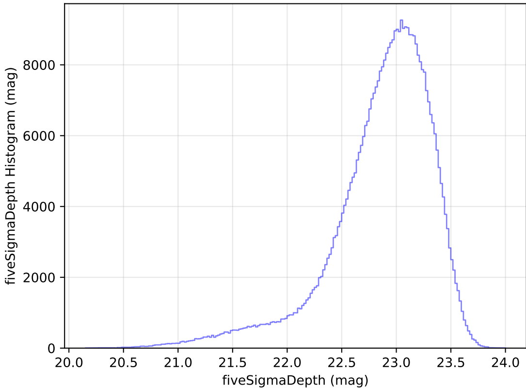
too_ignore_100_1v3.4_10yrs z: fiveSigmaDepth Histogram
