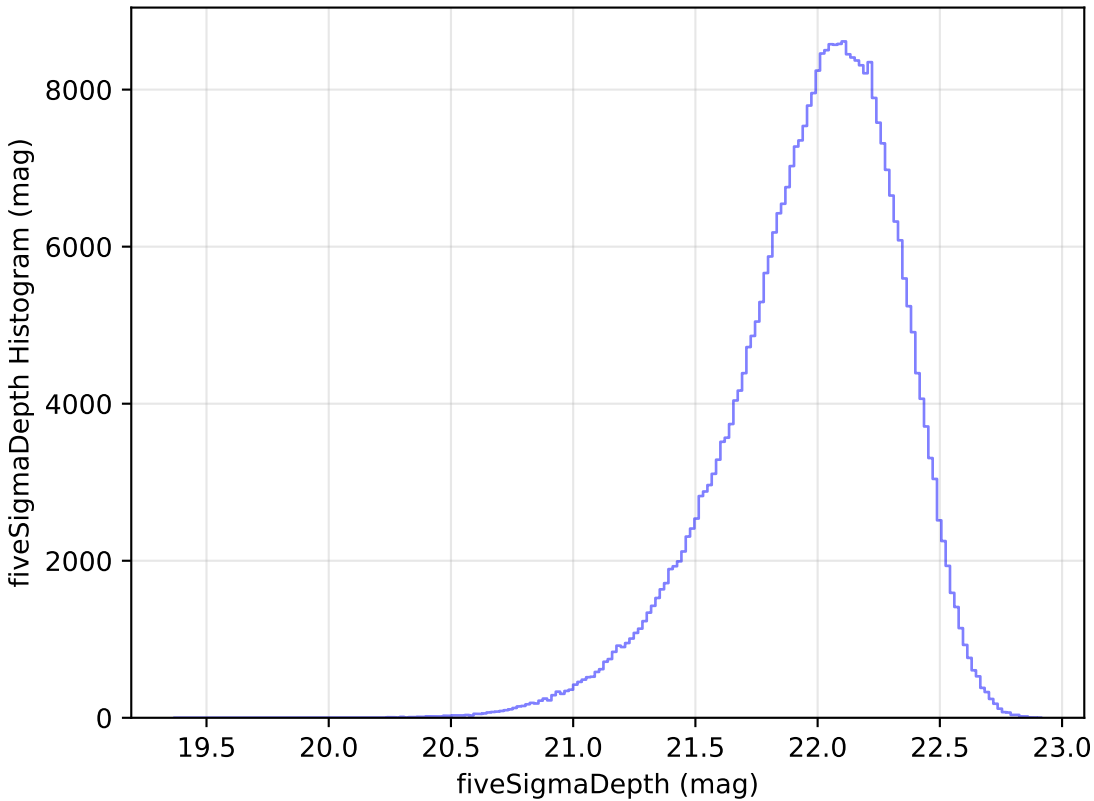
too_ignore_100_1v3.4_10yrs y: fiveSigmaDepth Histogram
