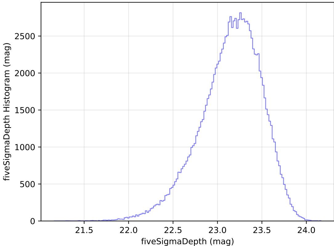
too_ignore_100_1v3.4_10yrs u: fiveSigmaDepth Histogram
