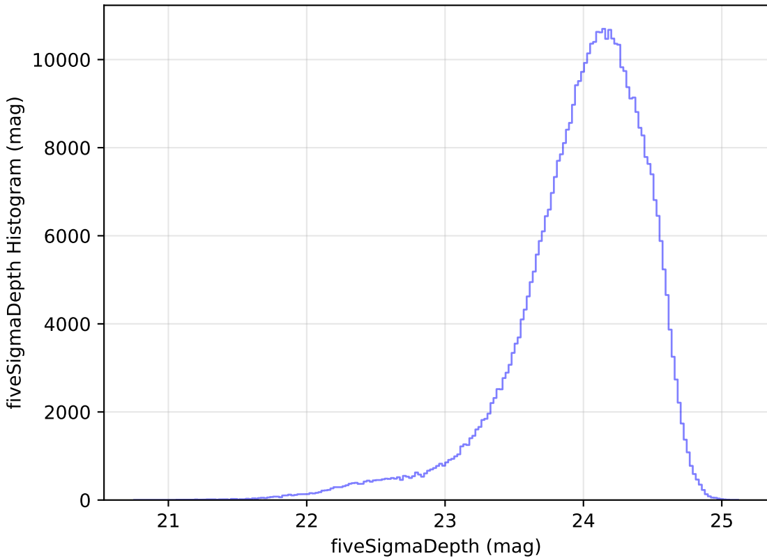
too_ignore_100_1v3.4_10yrs r: fiveSigmaDepth Histogram
