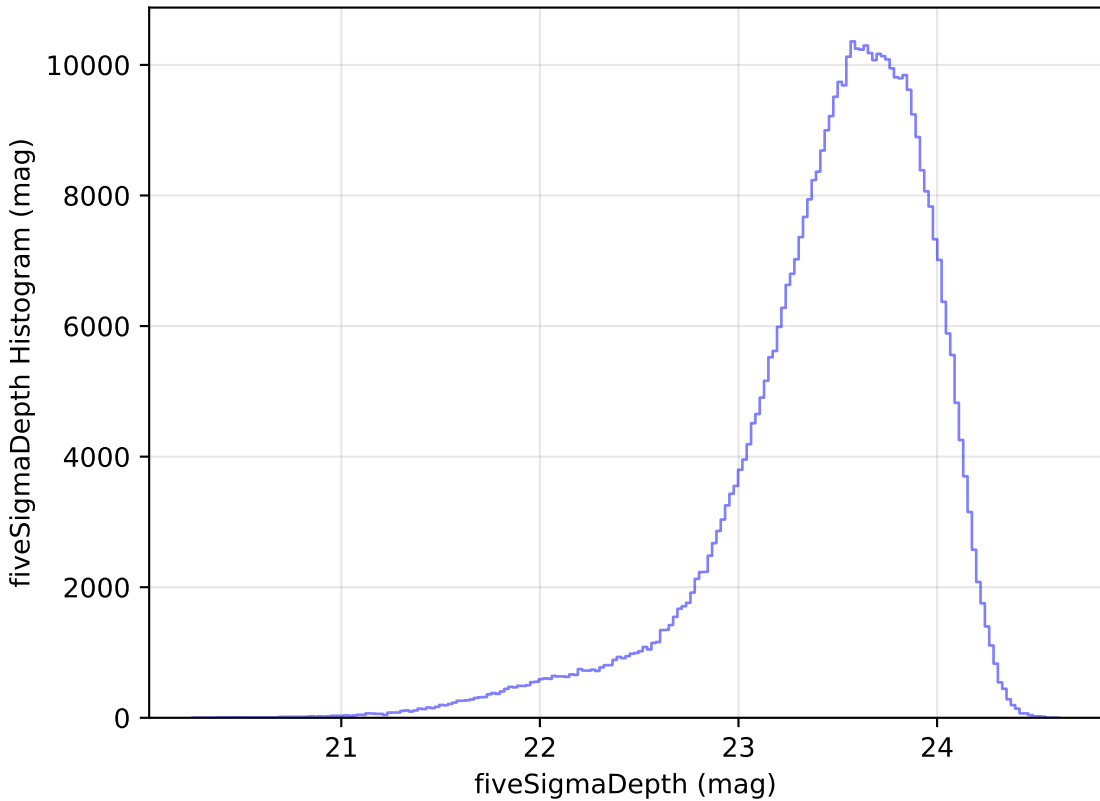
too_ignore_100_1v3.4_10yrs i: fiveSigmaDepth Histogram
