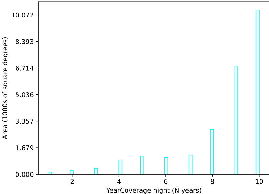
too_ignore_100_1v3.4_10yrs u band: YearCoverage night
