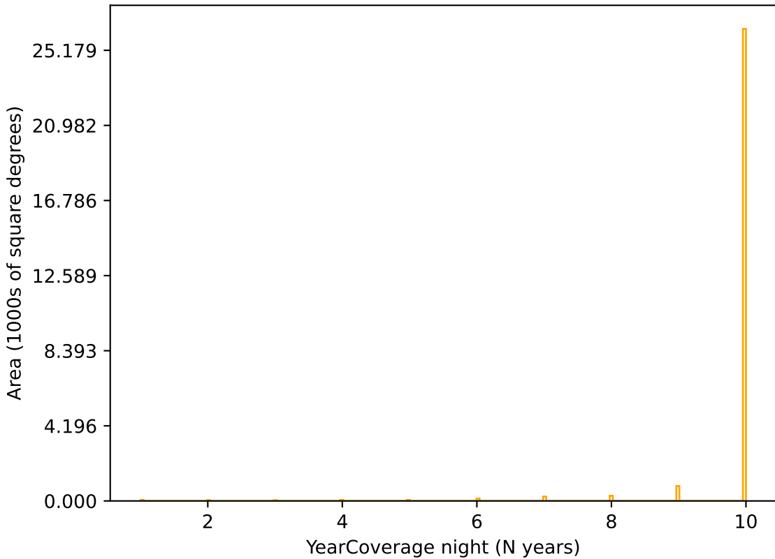
too_ignore_100_1v3.4_10yrs r band: YearCoverage night
