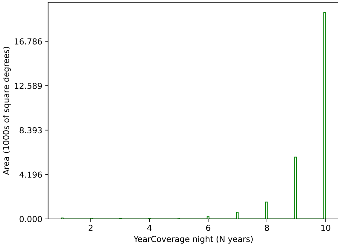
too_ignore_100_1v3.4_10yrs g band: YearCoverage night
