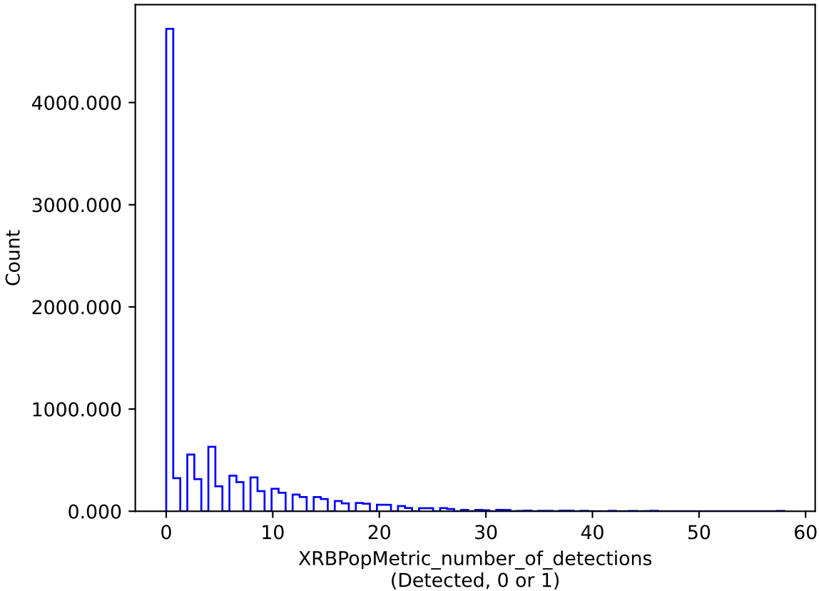
too_ignore_100_1v3.4_10yrs : XRBPoMetric_number_of_detections
