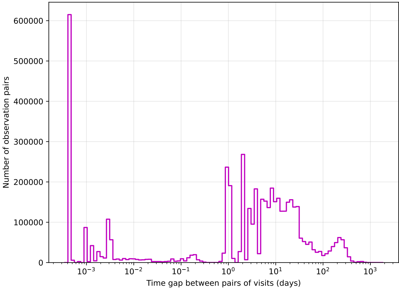
too_ignore_100_1v3.4_10yrs z band: Tgaps observationStartMJD
