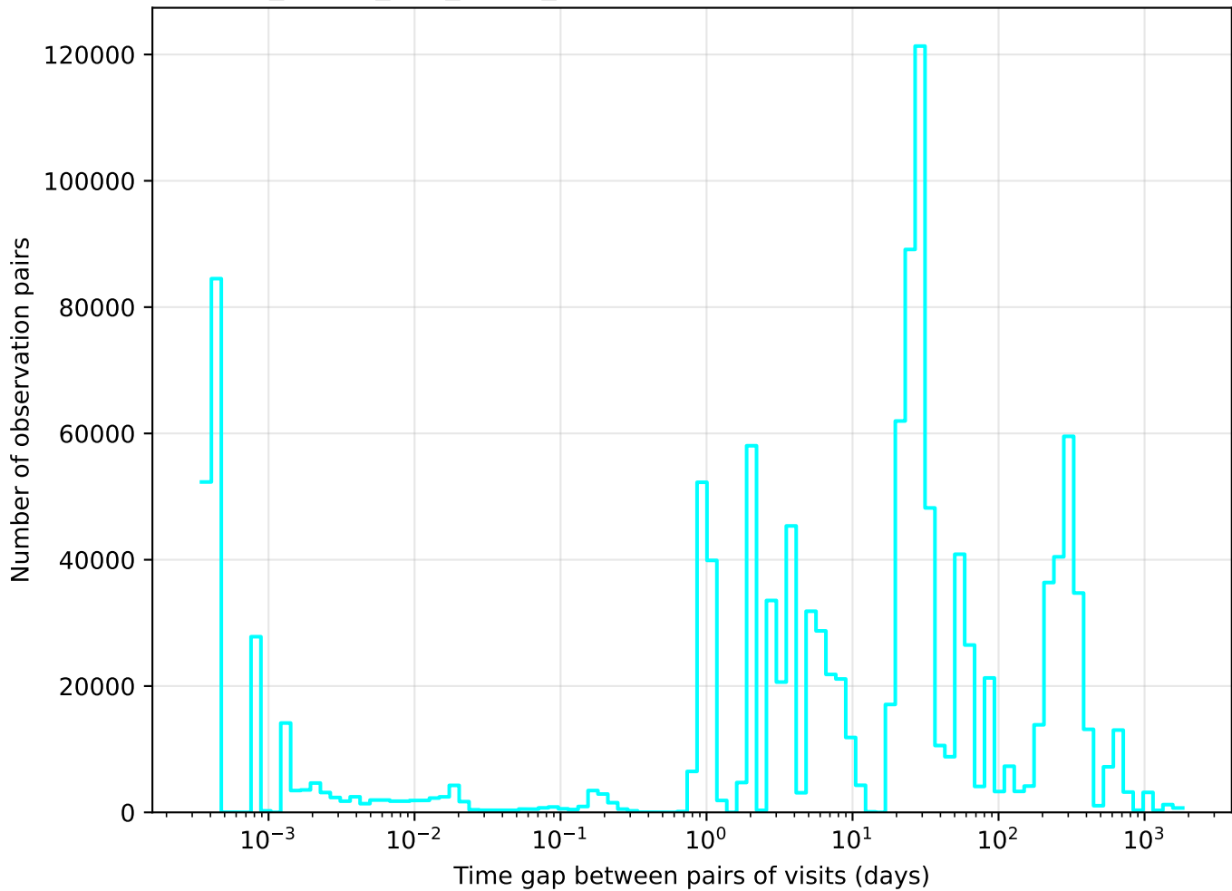
too_ignore_100_1v3.4_10yrs u band: Tgaps observationStartMJD
