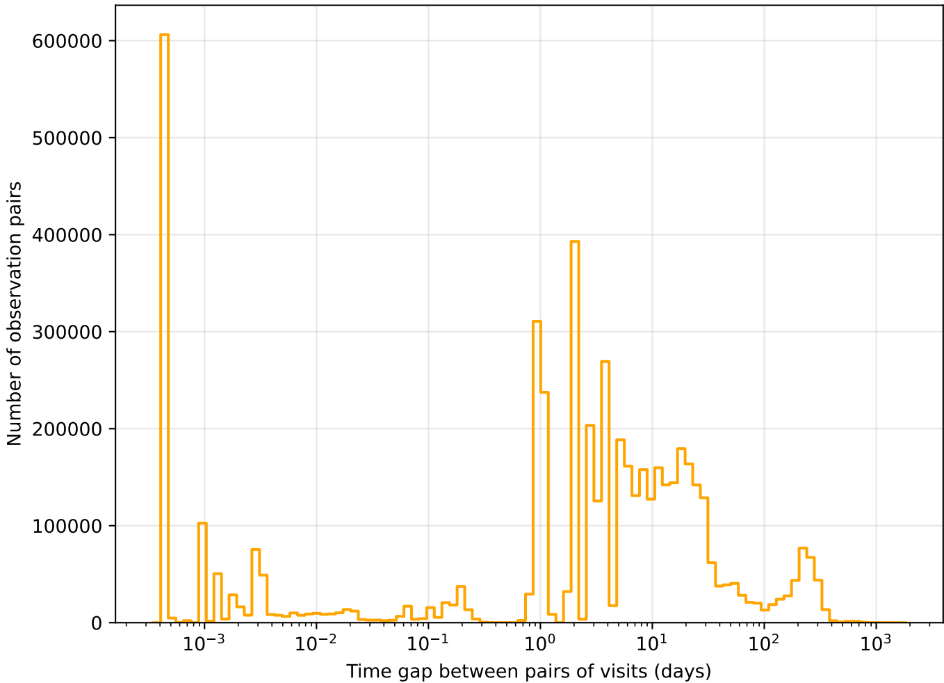
too_ignore_100_1v3.4_10yrs r band: Tgaps observationStartMJD
