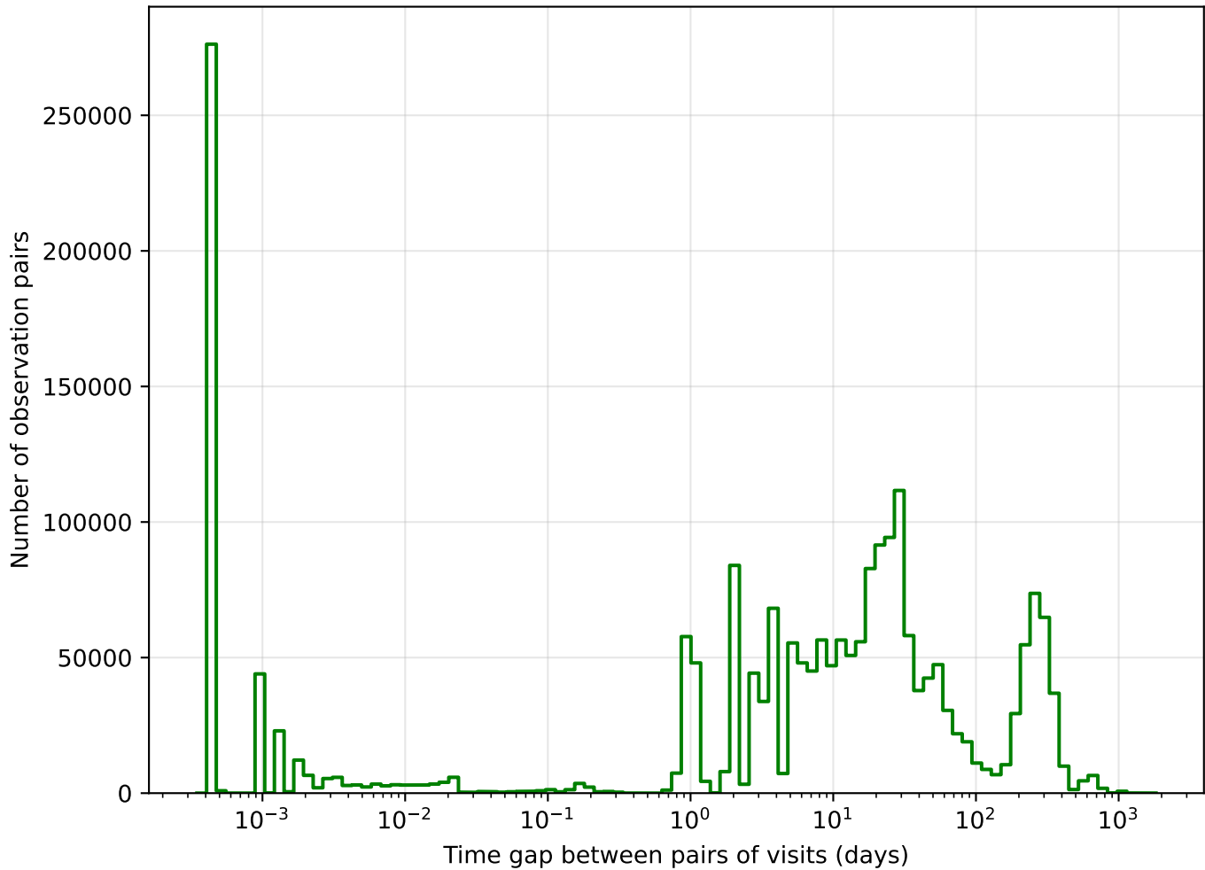
too_ignore_100_1v3.4_10yrs g band: Tgaps observationStartMJD
