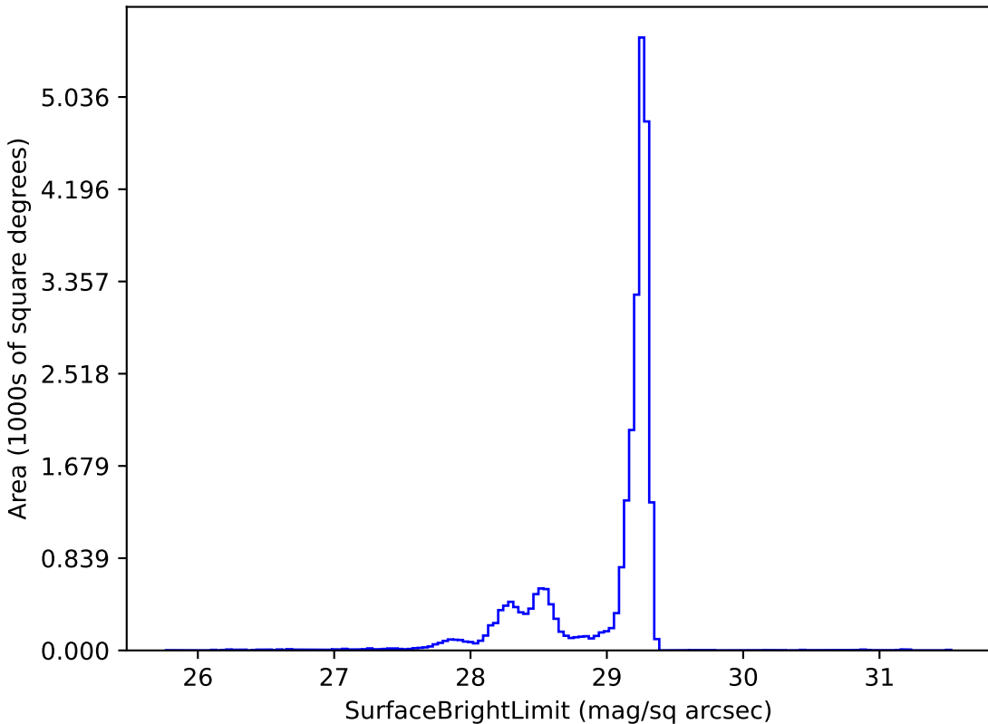
too_ignore_100_1v3.4_10yrs z: SurfaceBrightLimit
