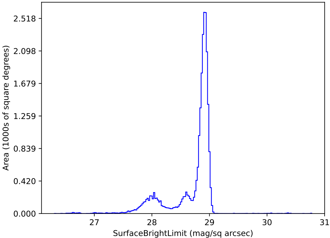
too_ignore_100_1v3.4_10yrs u: SurfaceBrightLimit
