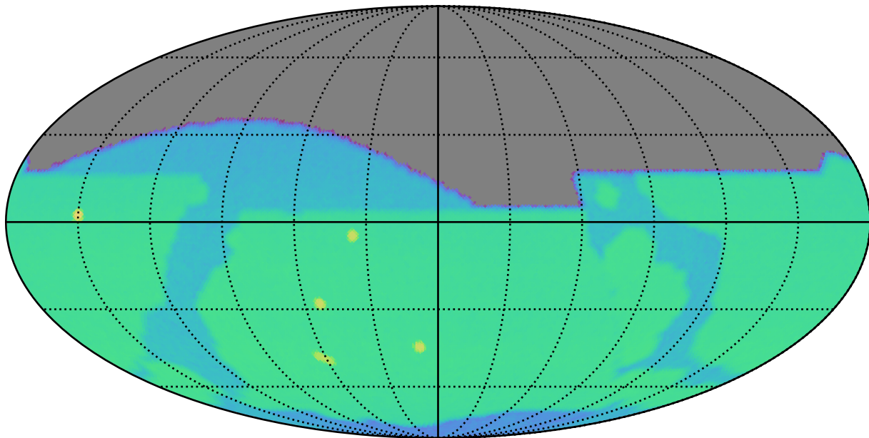
too_ignore_100_1v3.4_10yrs r: SurfaceBrightLimit
