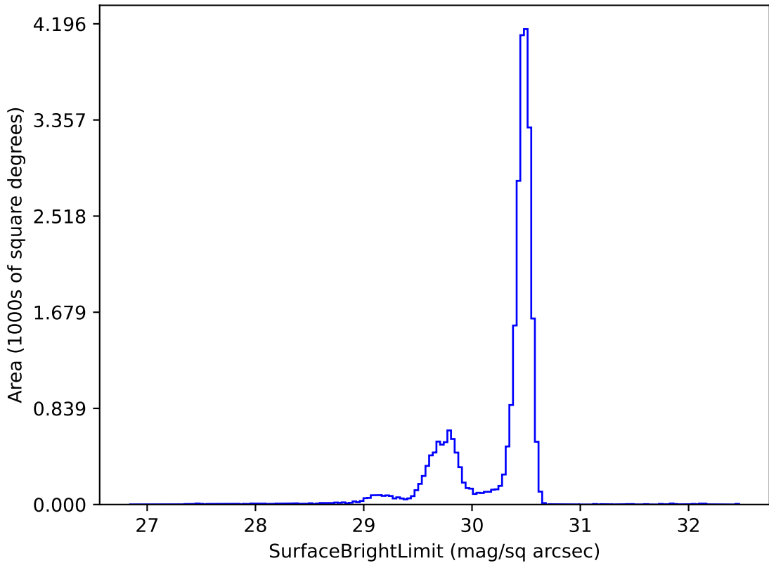
too_ignore_100_1v3.4_10yrs r: SurfaceBrightLimit
