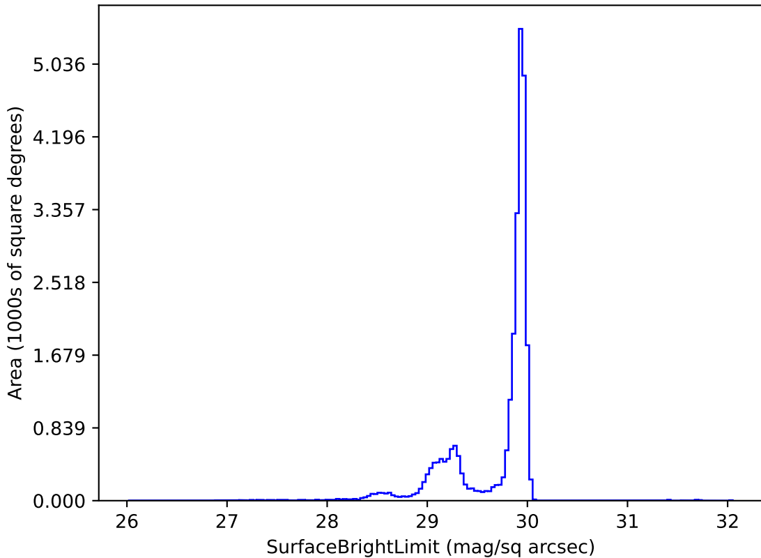
too_ignore_100_1v3.4_10yrs i: SurfaceBrightLimit
