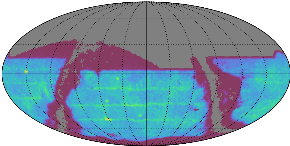
too_ignore_100_1v3.4_10yrs : SNSLMetric
