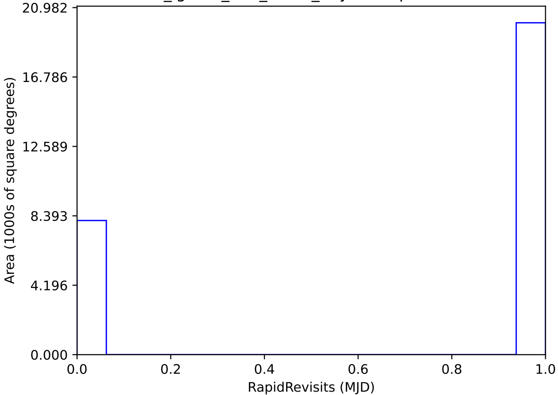
too_ignore_100_1v3.4_10yrs : RapidRevisits
