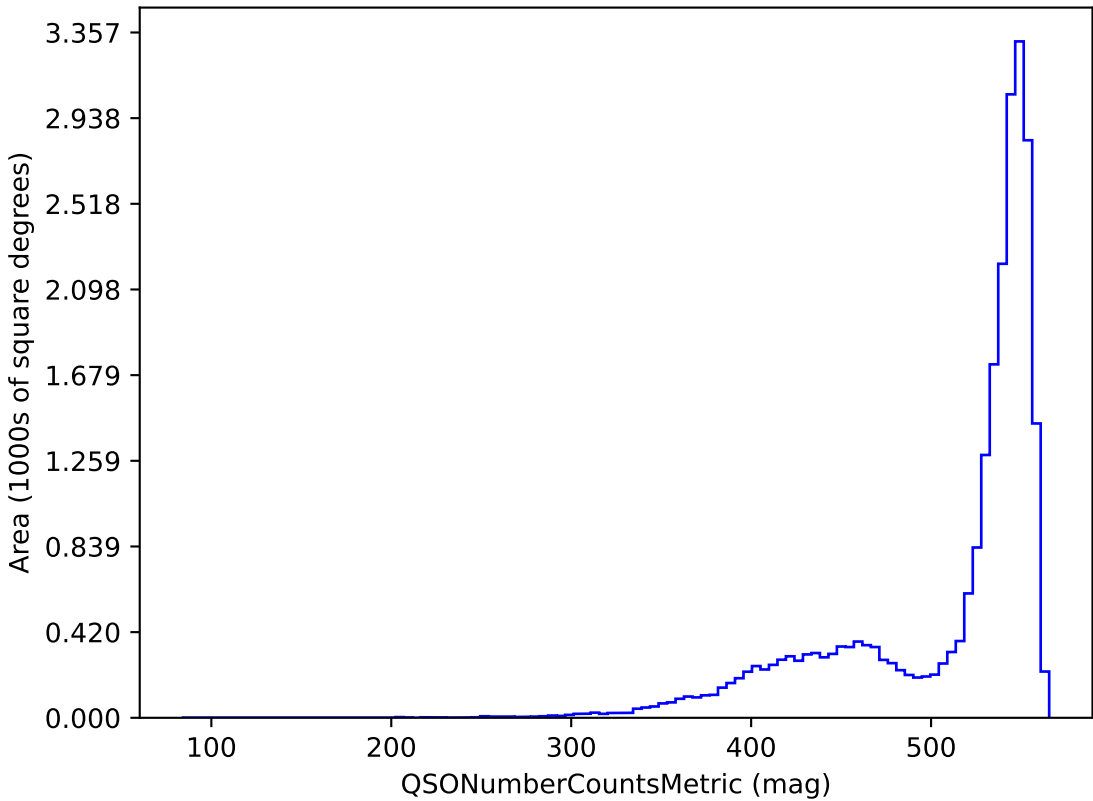
too_ignore_100_1v3.4_10yrs i band and non-DD: QSONumberCountsMetric
