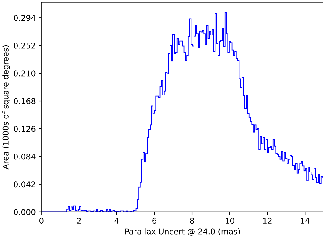
too_ignore_100_1v3.4_10yrs : Parallax Uncert @ 24.0
