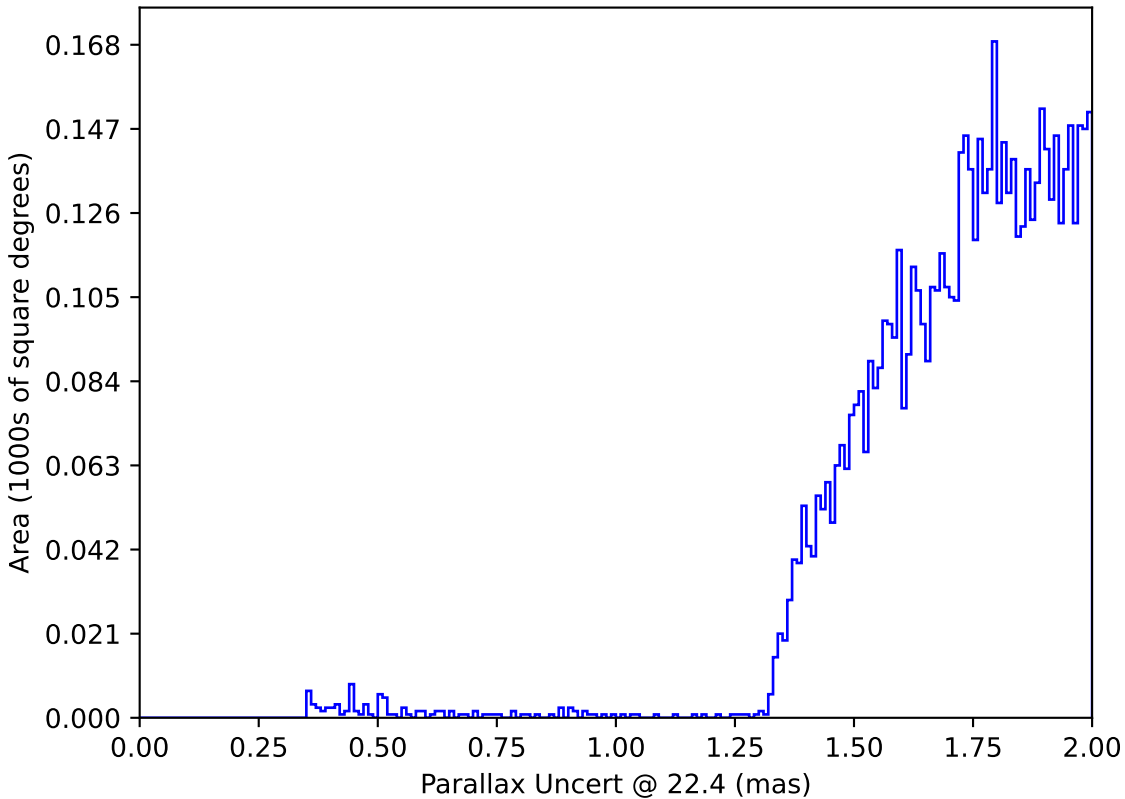
too_ignore_100_1v3.4_10yrs : Parallax Uncert @ 22.4
