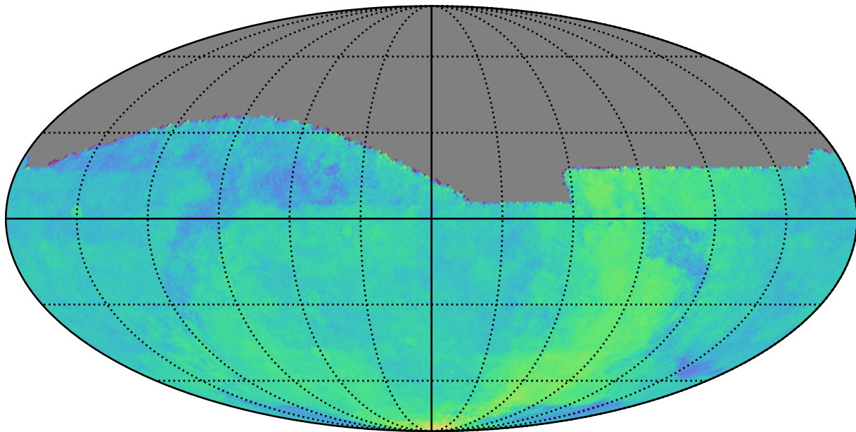
too_ignore_100_1v3.4_10yrs : Parallax Coverage @ 24.0
