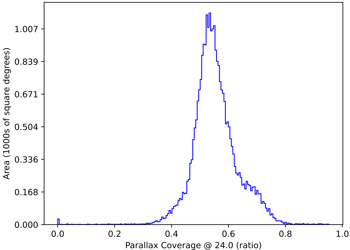
too_ignore_100_1v3.4_10yrs : Parallax Coverage @ 24.0
