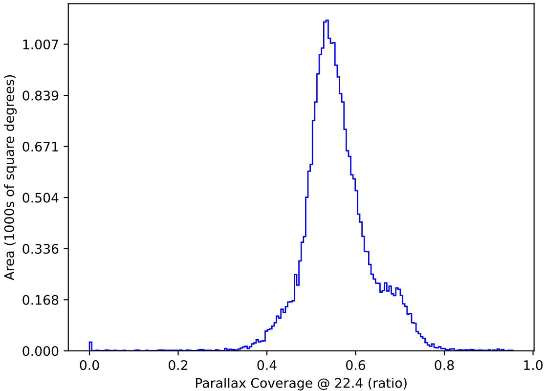
too_ignore_100_1v3.4_10yrs : Parallax Coverage @ 22.4
