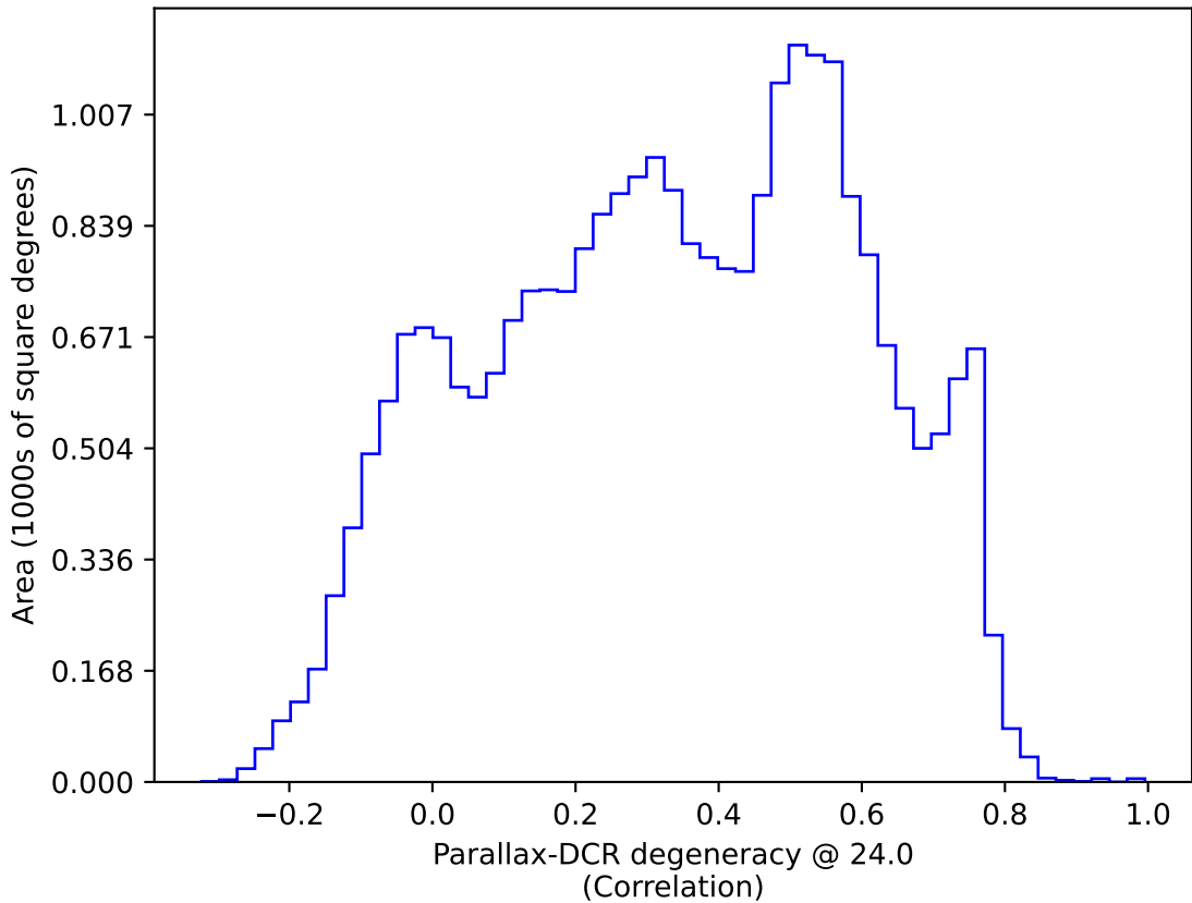
too_ignore_100_1v3.4_10yrs : Parallax-DCR degeneracy @ 24.0
