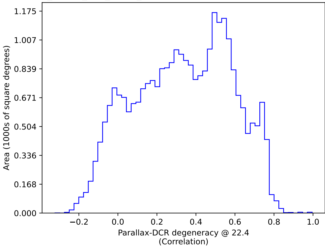
too_ignore_100_1v3.4_10yrs : Parallax-DCR degeneracy @ 22.4
