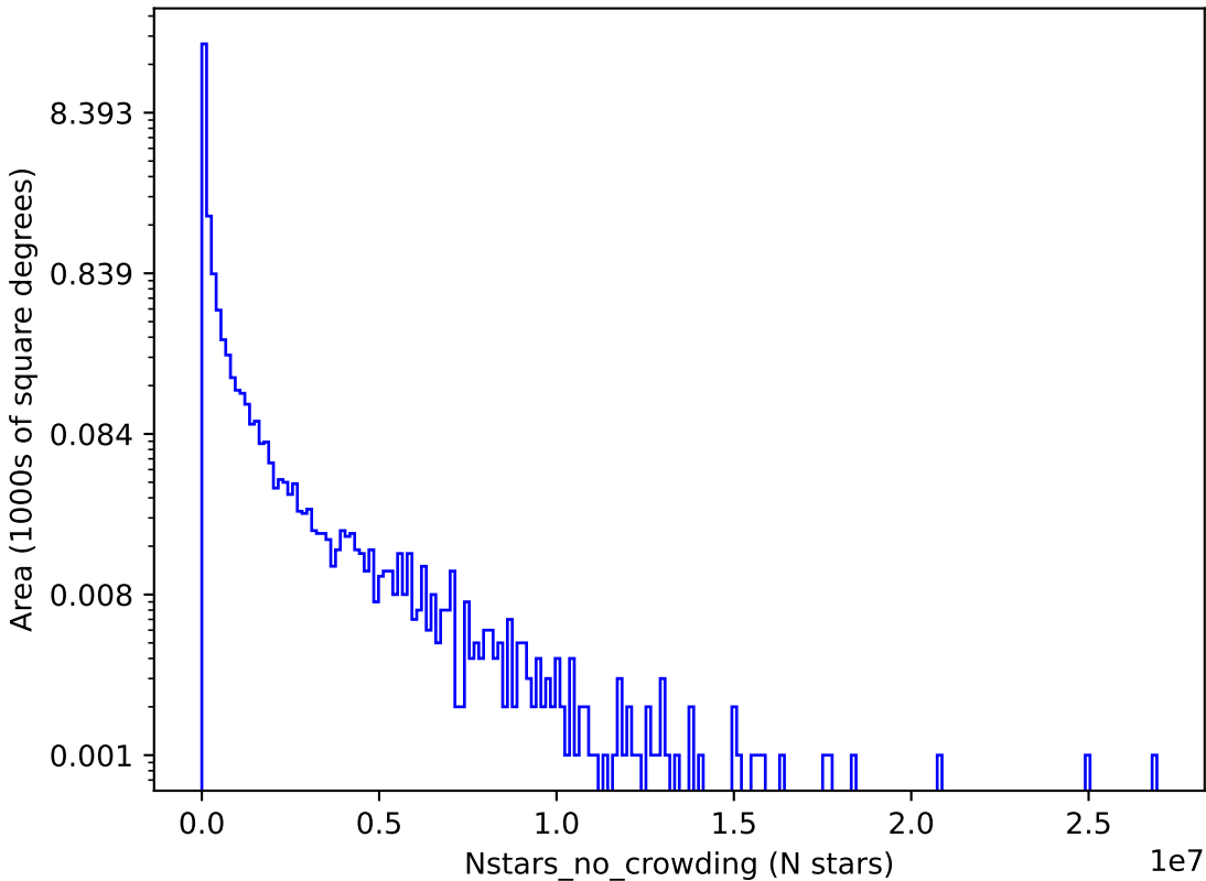
too_ignore_100_1v3.4_10yrs z: Nstars_no_crowding
