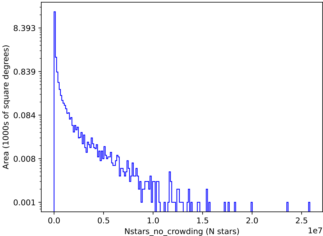
too_ignore_100_1v3.4_10yrs y: Nstars_no_crowding
