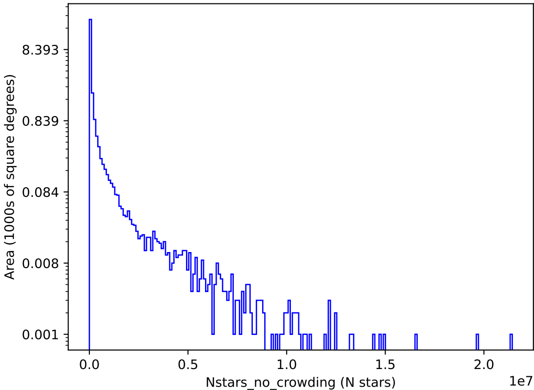
too_ignore_100_1v3.4_10yrs r: Nstars_no_crowding
