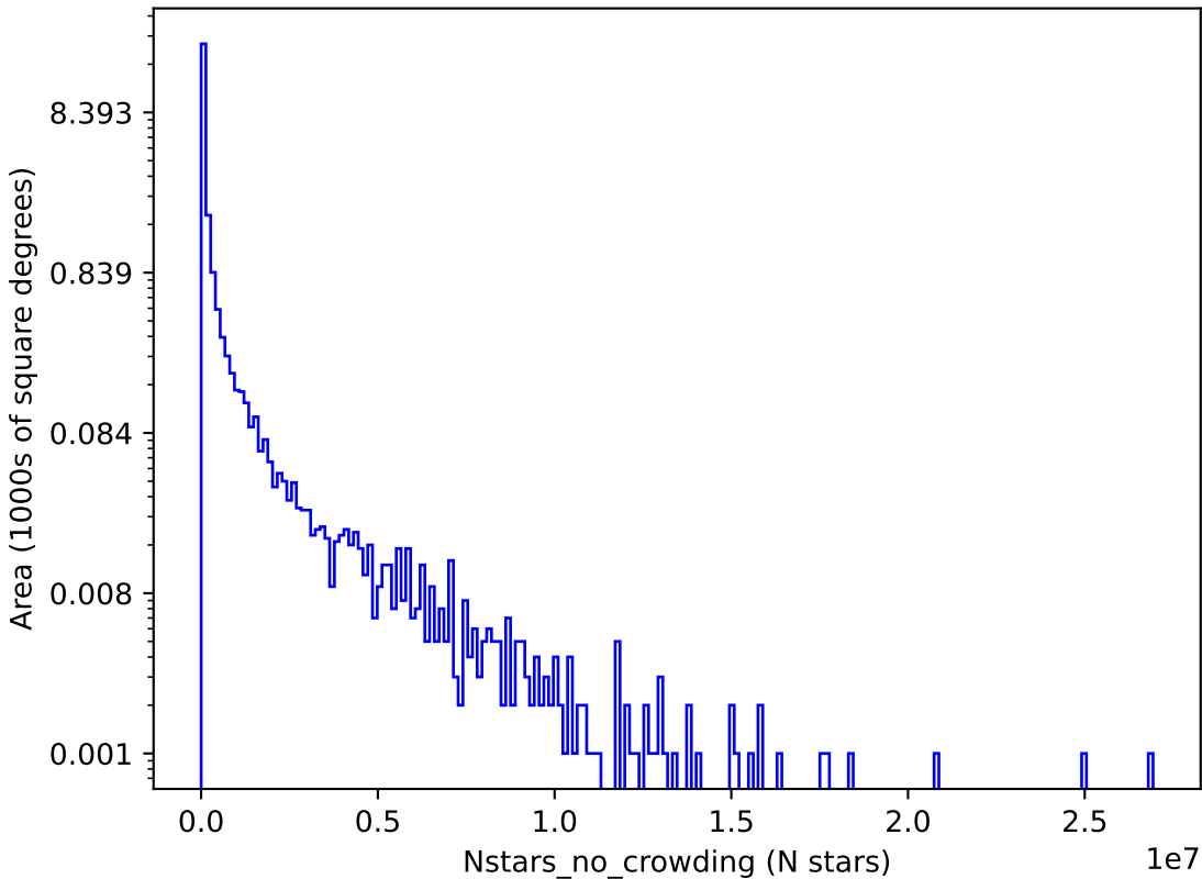
too_ignore_100_1v3.4_10yrs i: Nstars_no_crowding
