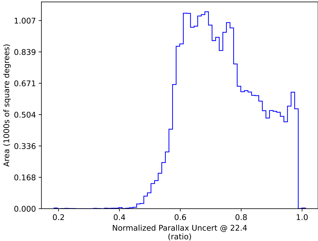
too_ignore_100_1v3.4_10yrs : Normalized Parallax Uncert @ 22.4
