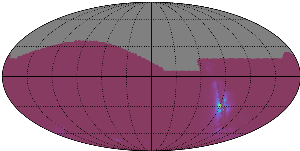
too_ignore_100_1v3.4_10yrs : NlcPoints
