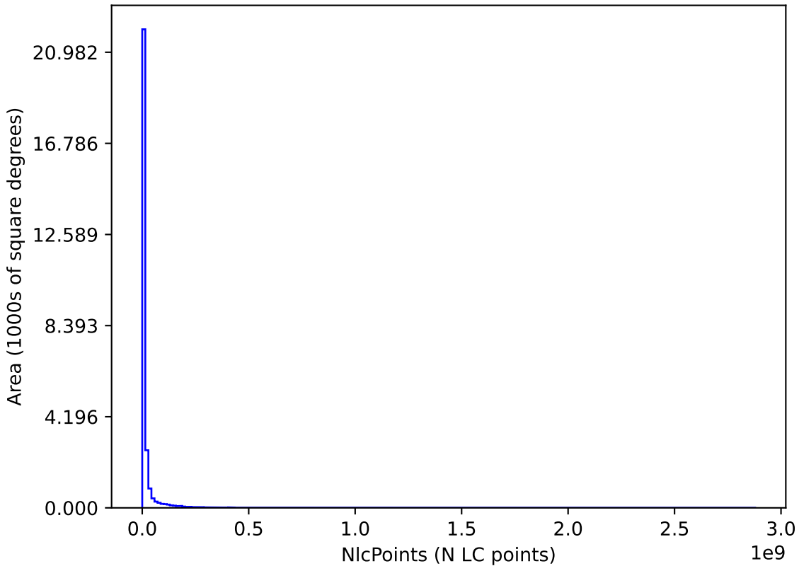
too_ignore_100_1v3.4_10yrs : NlcPoints
