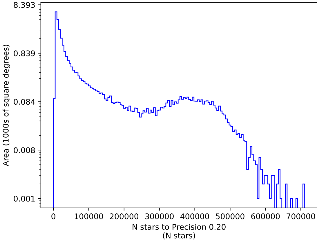
too_ignore_100_1v3.4_10yrs z: N stars to Precision 0.20
